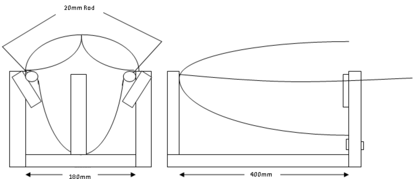
Figure 3 - Detail of approved ILS Jig for measuring reverse curve of Ski (NOT TO SCALE)
